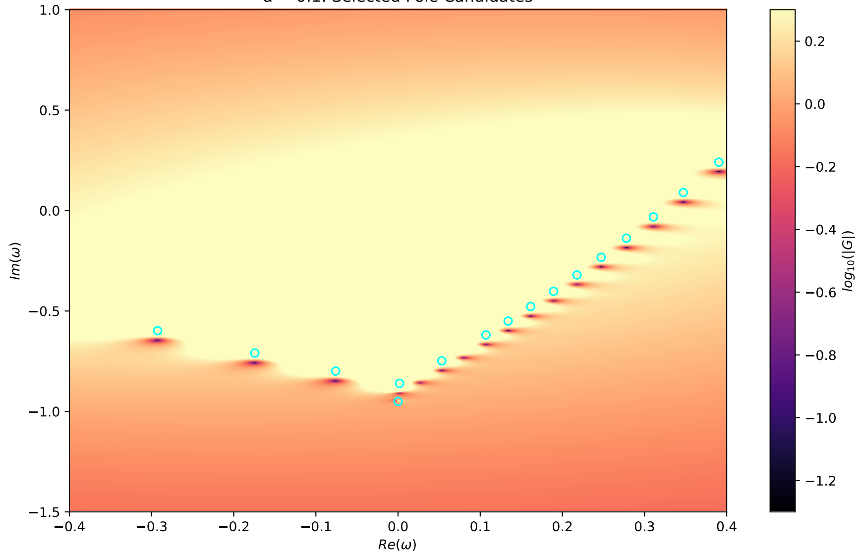
a = 0.1 : Selected Pole Candidates
