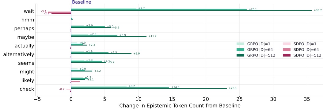
Figure 11: Change in epistemic token counts relative to the base model on AIME24 for GRPO and SDPO with |D| \in \{1, 64, 512\} .
