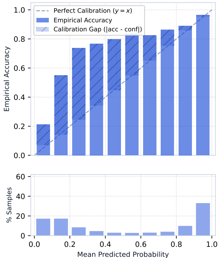
(b) Affine Platt Scaled ( T_{\text{eff}} = 3.5931 )
