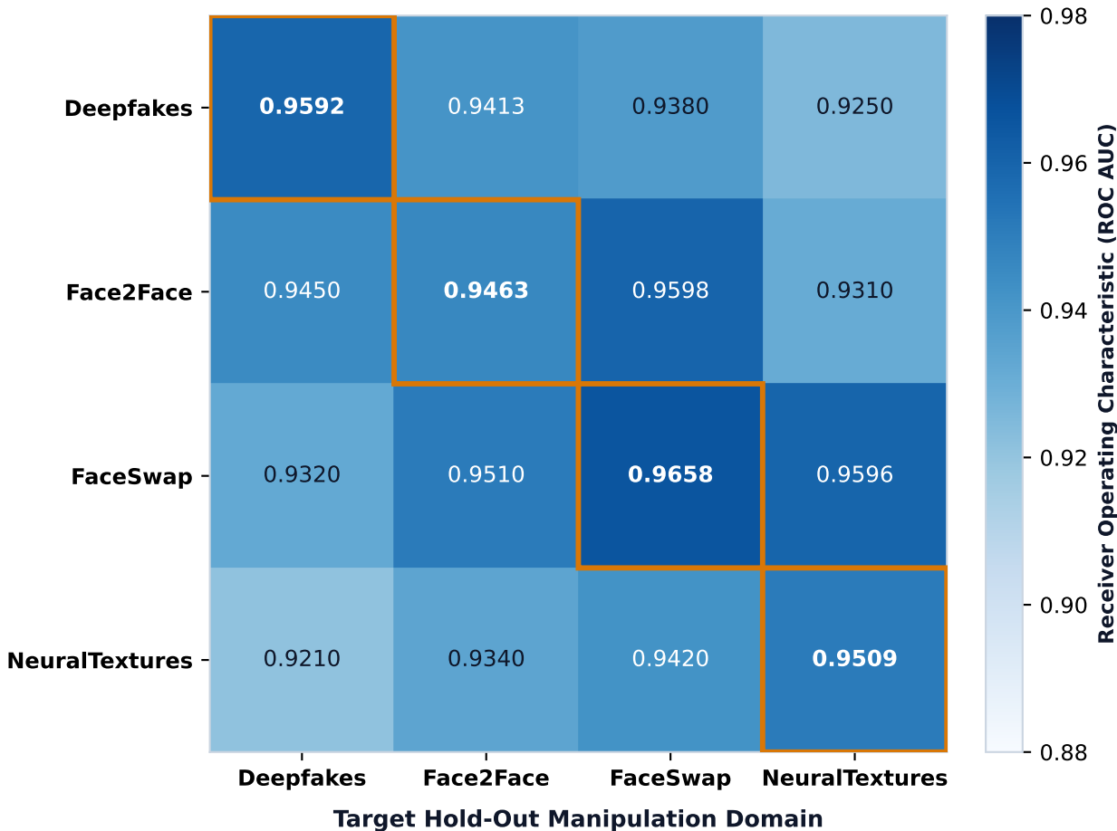
Leave-One-Type-Out (LOTO) Cross-Generator Generalization Matrix
