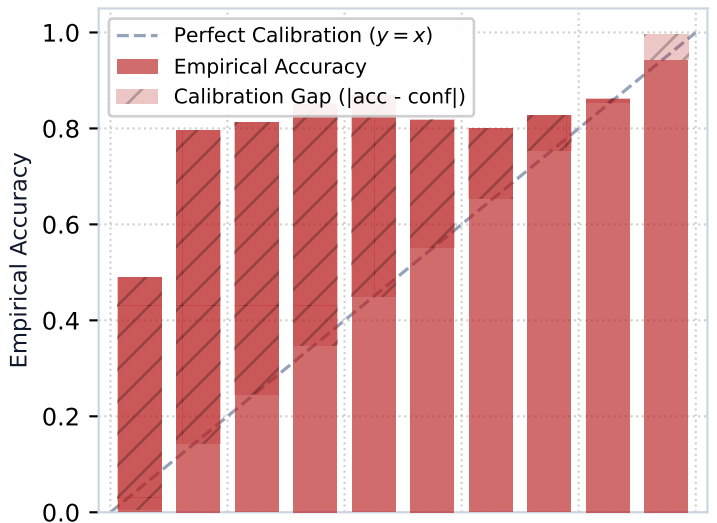
(a) Pre-Calibration Overconfidence
