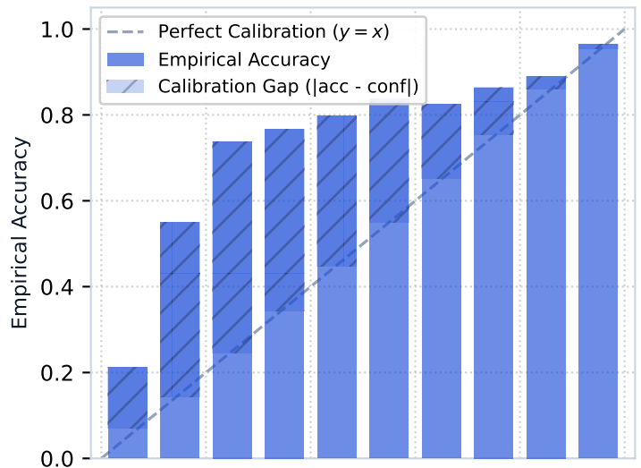
(b) Affine Platt Scaled ( T_{\text{eff}} = 3.5931 )
