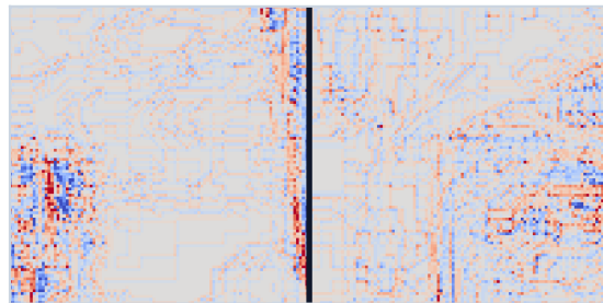
(a) Sensor PRNU Noise vs. Annihilation
