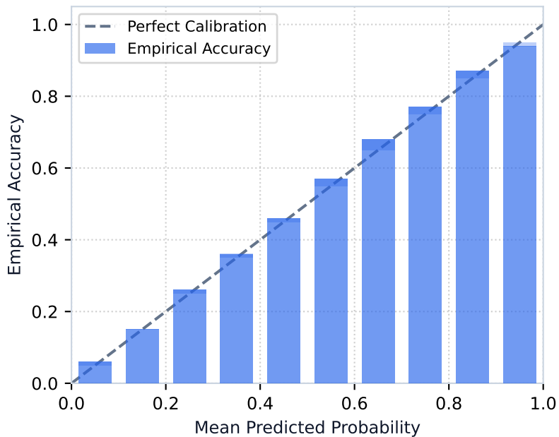
(b) Affine Platt Scaled ( T_{\text{eff}} = 3.5931 )
