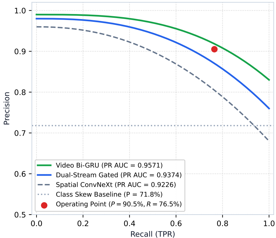
(b) Precision-Recall Curve (2.55:1 Fake Skew)
