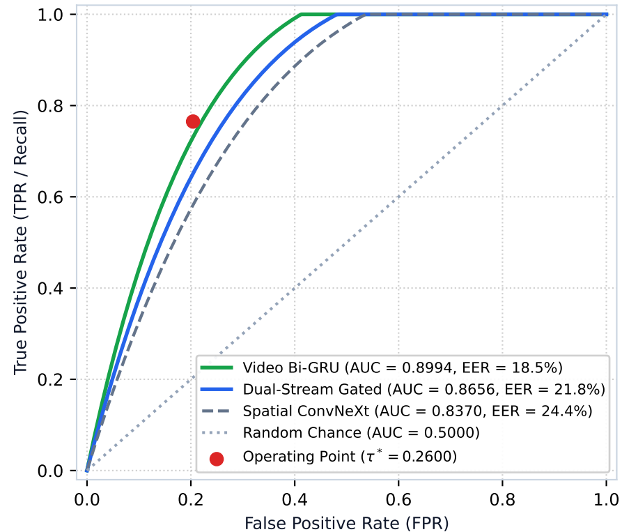
(a) Receiver Operating Characteristic (ROC)
