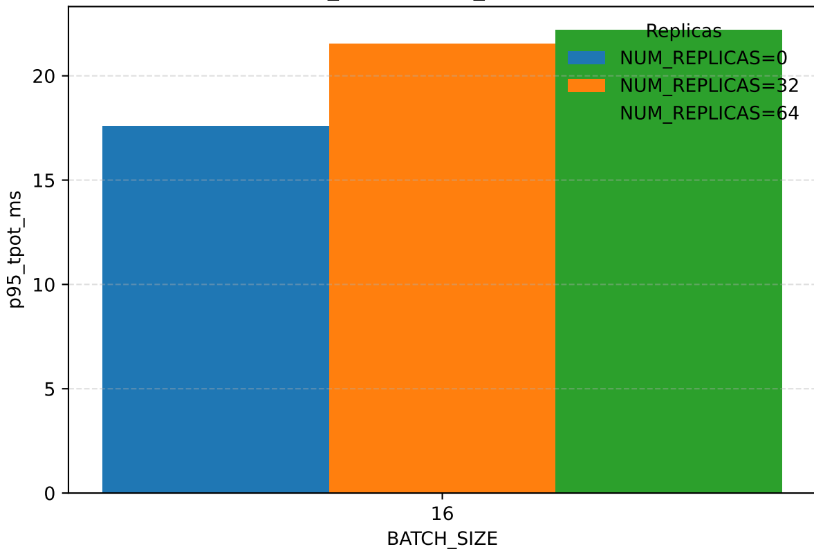
p95_tpot_ms vs BATCH_SIZE NUM_GPUS=8, EP_DEGREE=8
