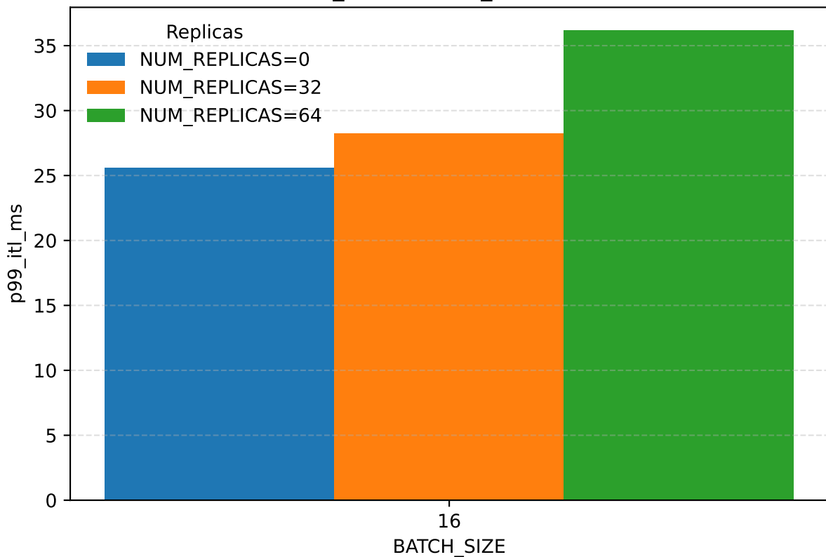
p99_itl_ms vs BATCH_SIZE NUM_GPUS=8, EP_DEGREE=8
