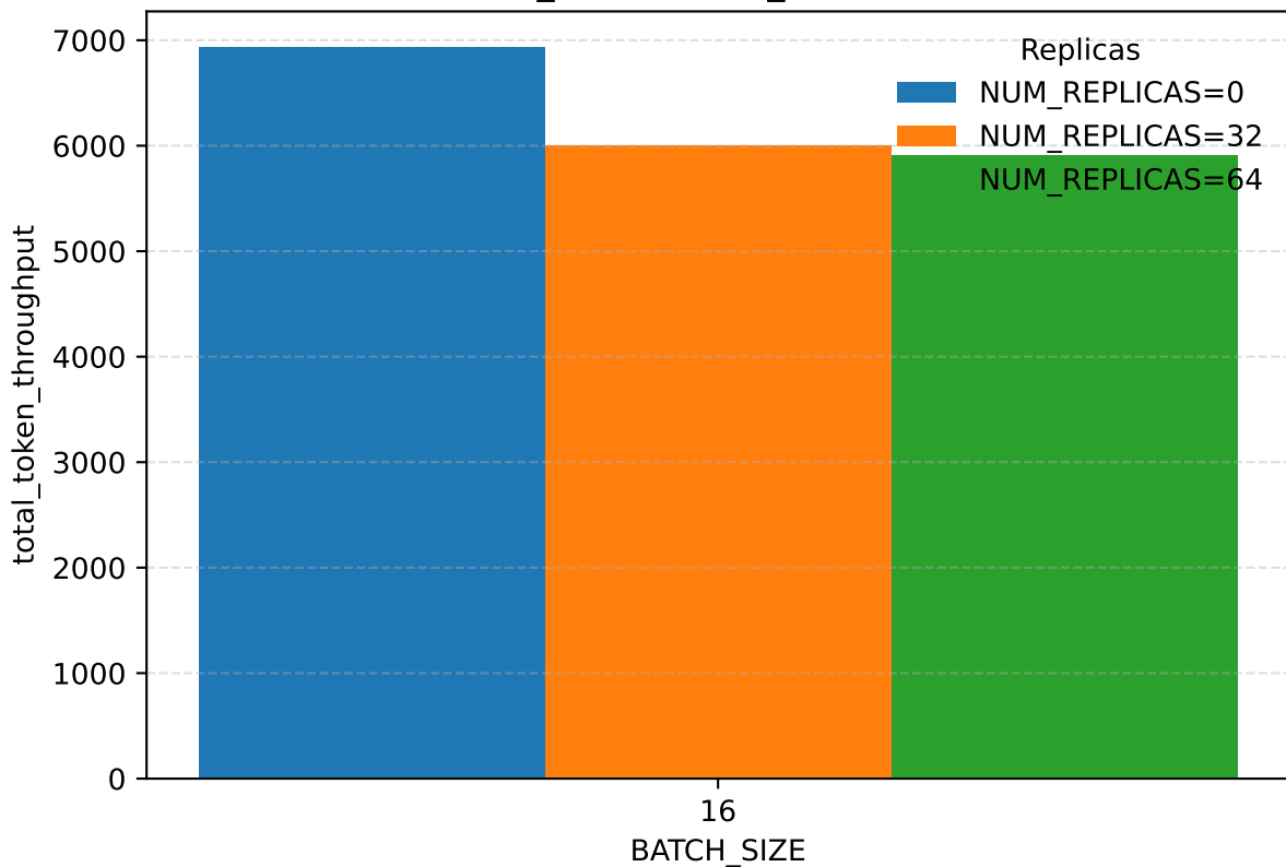
total_token_throughput vs BATCH_SIZE NUM_GPUS=8, EP_DEGREE=8
