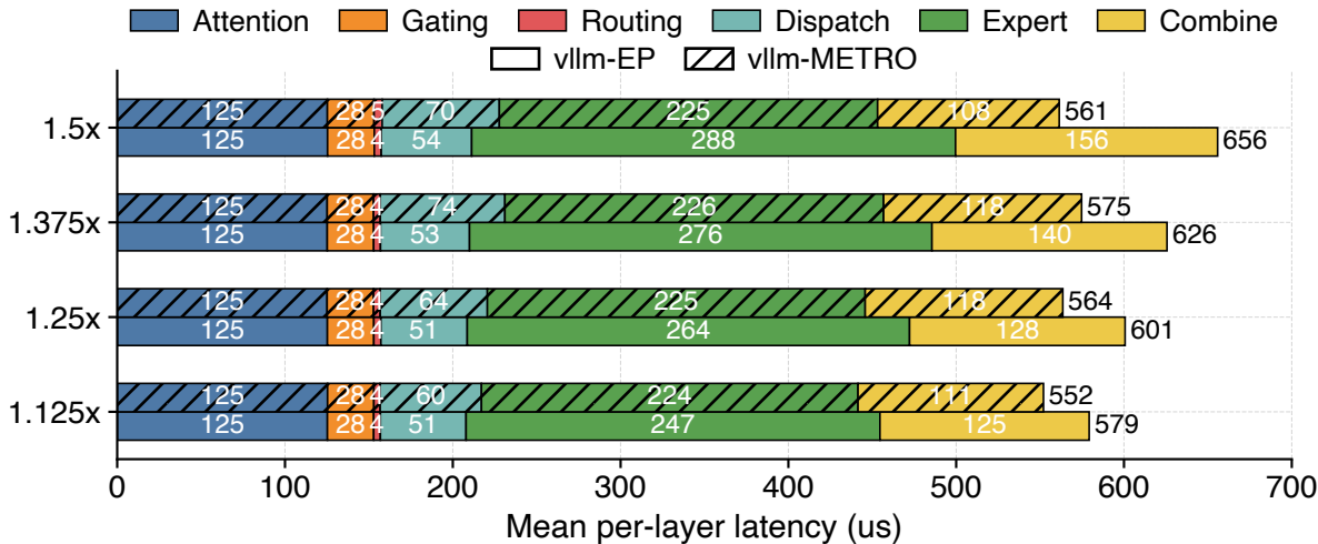
Replication Ratio
