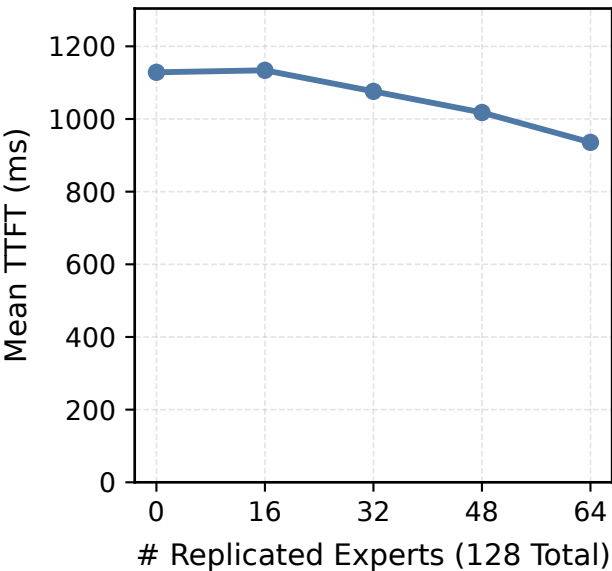
Prefill Latency
