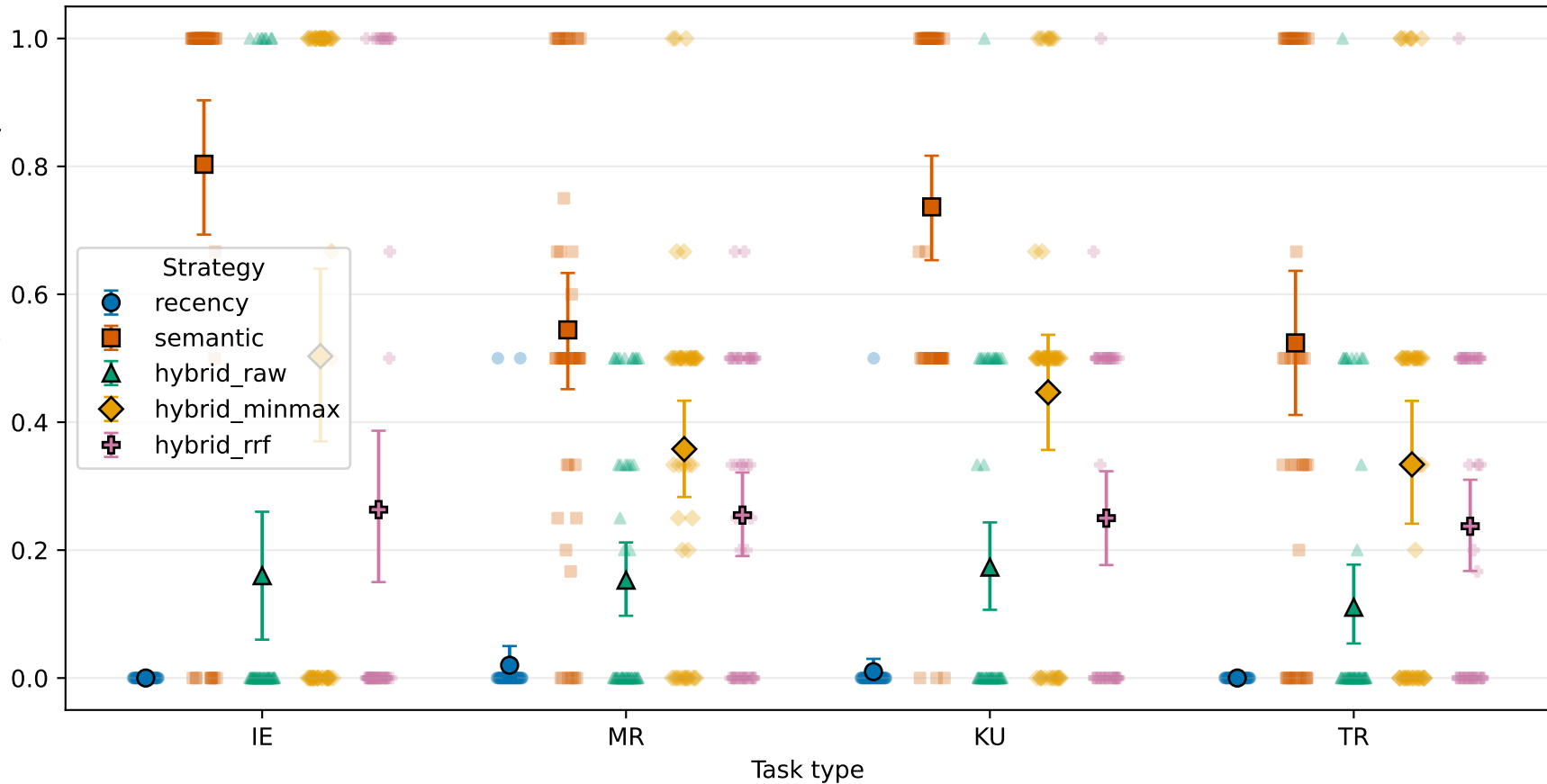
Mean round-level Recall@5 (95% bootstrap CI)
