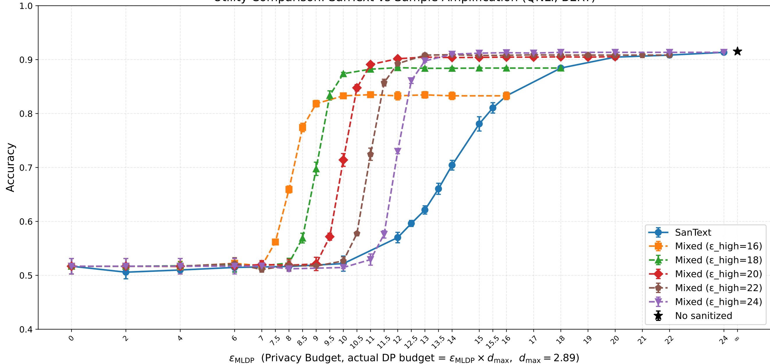
Utility Comparison: SanText vs Sample Amplification (QNLI, BERT)
