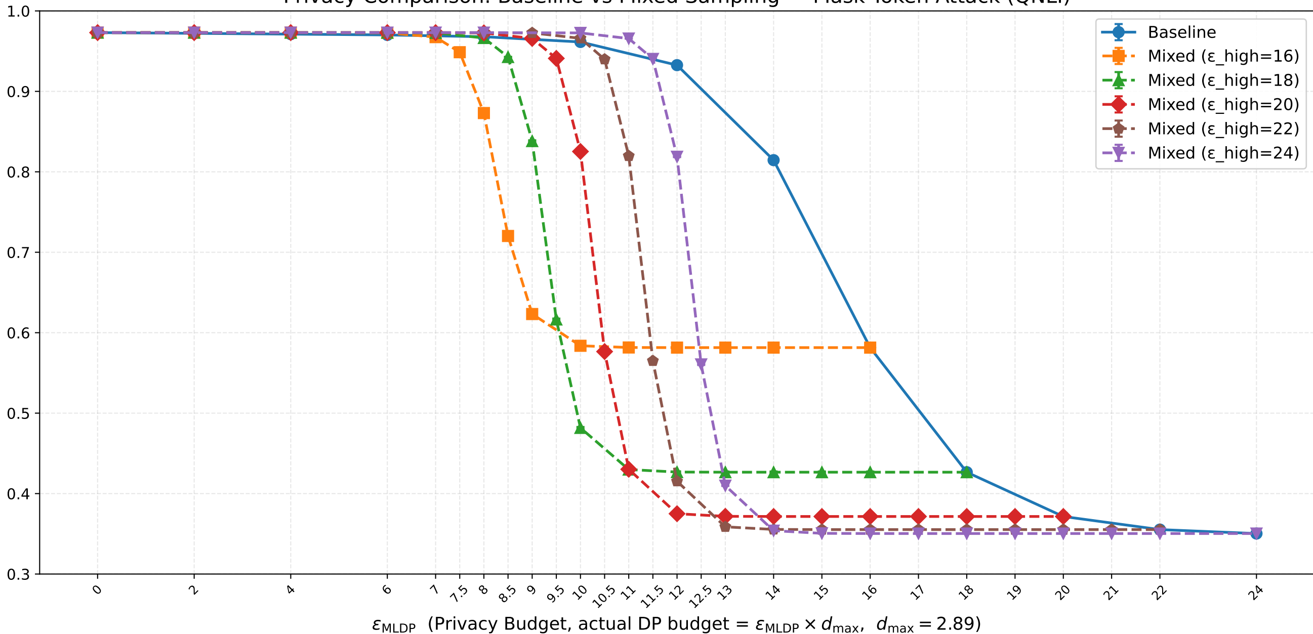
Privacy Comparison: Baseline vs Mixed Sampling — Mask Token Attack (QNLI)
