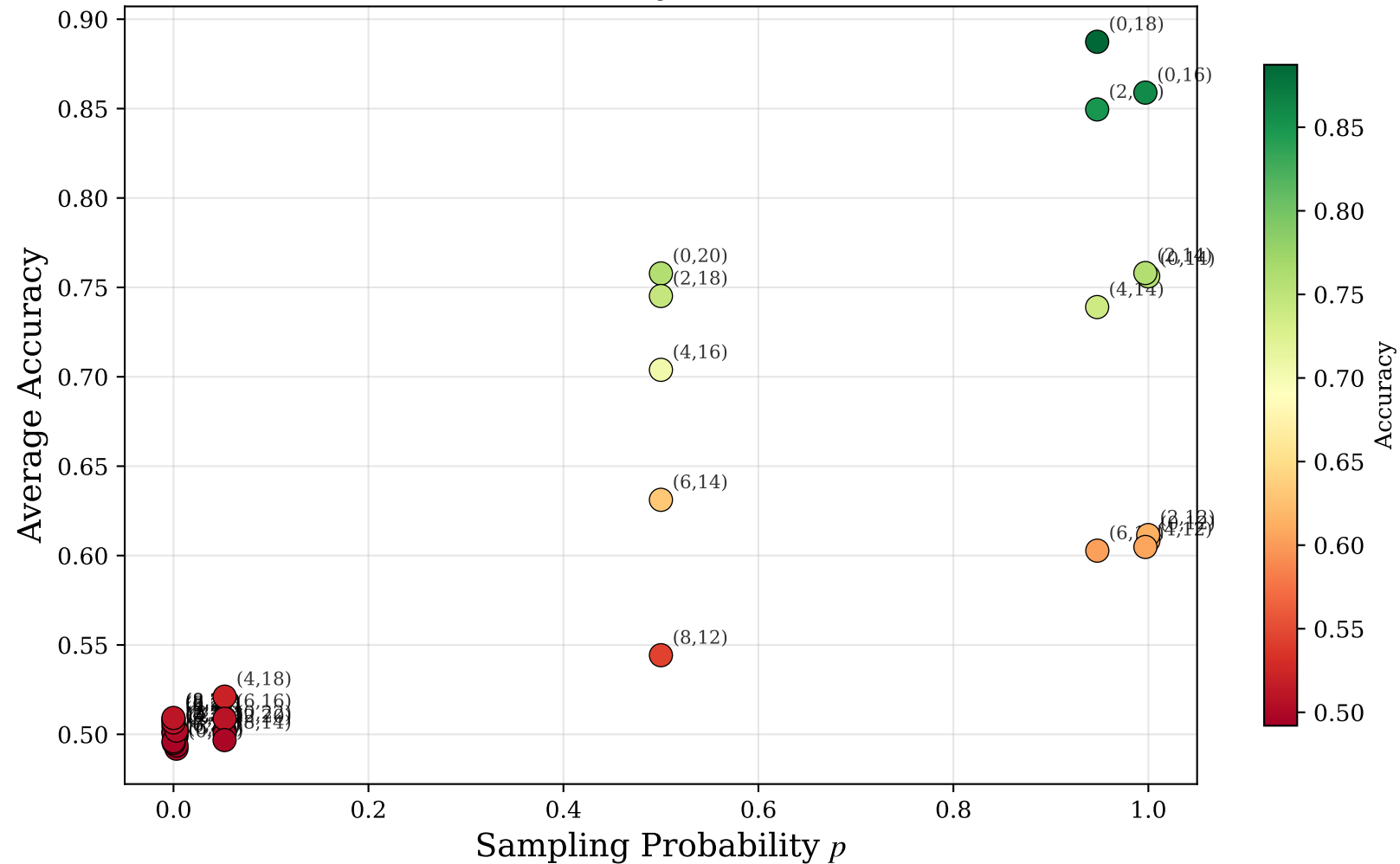
Accuracy vs Sampling Probability p (Fixed \varepsilon_{target} = 10.0 )
