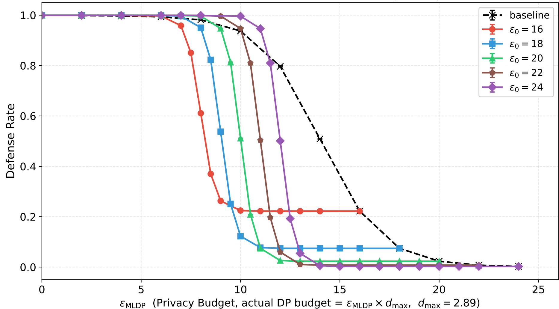
KNN Attack (Top-10) Defense Rate — QNLI, Sample Amplification
