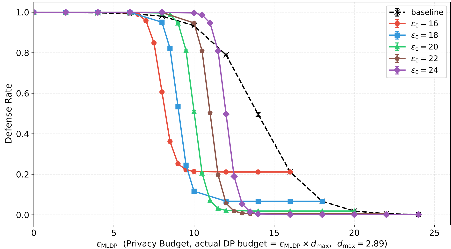
KNN Attack (Top-10) Defense Rate — SST2, Sample Amplification
