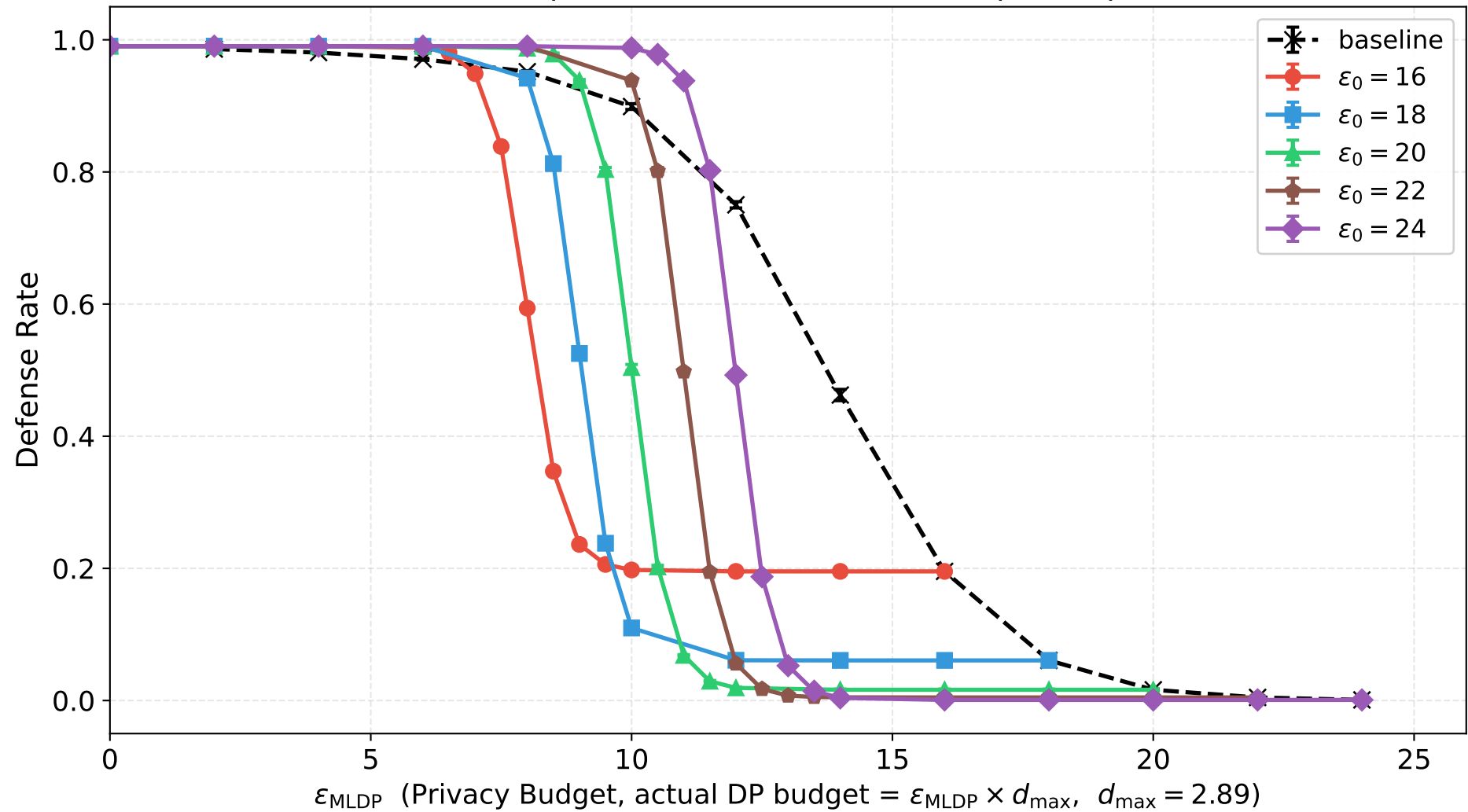
KNN Attack (Top-300) Defense Rate — Sample Amplification
