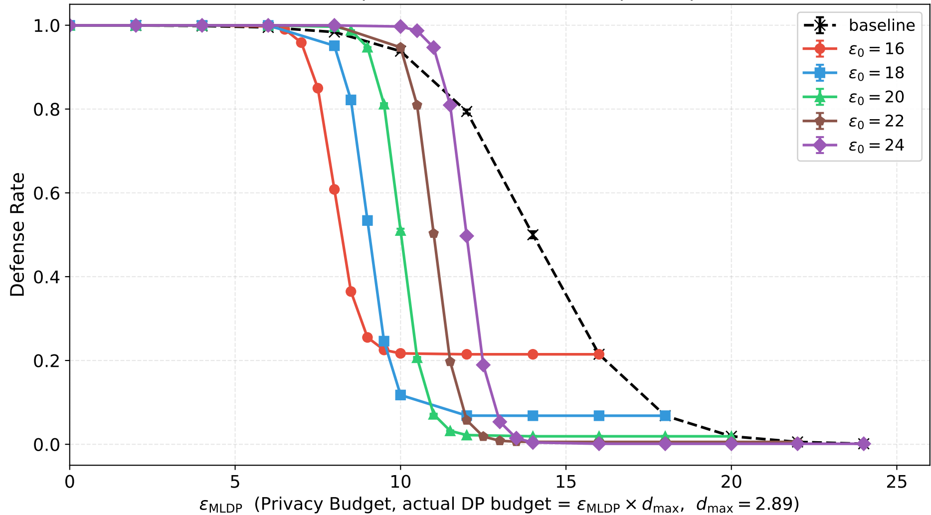
KNN Attack (Top-5) Defense Rate — Sample Amplification
