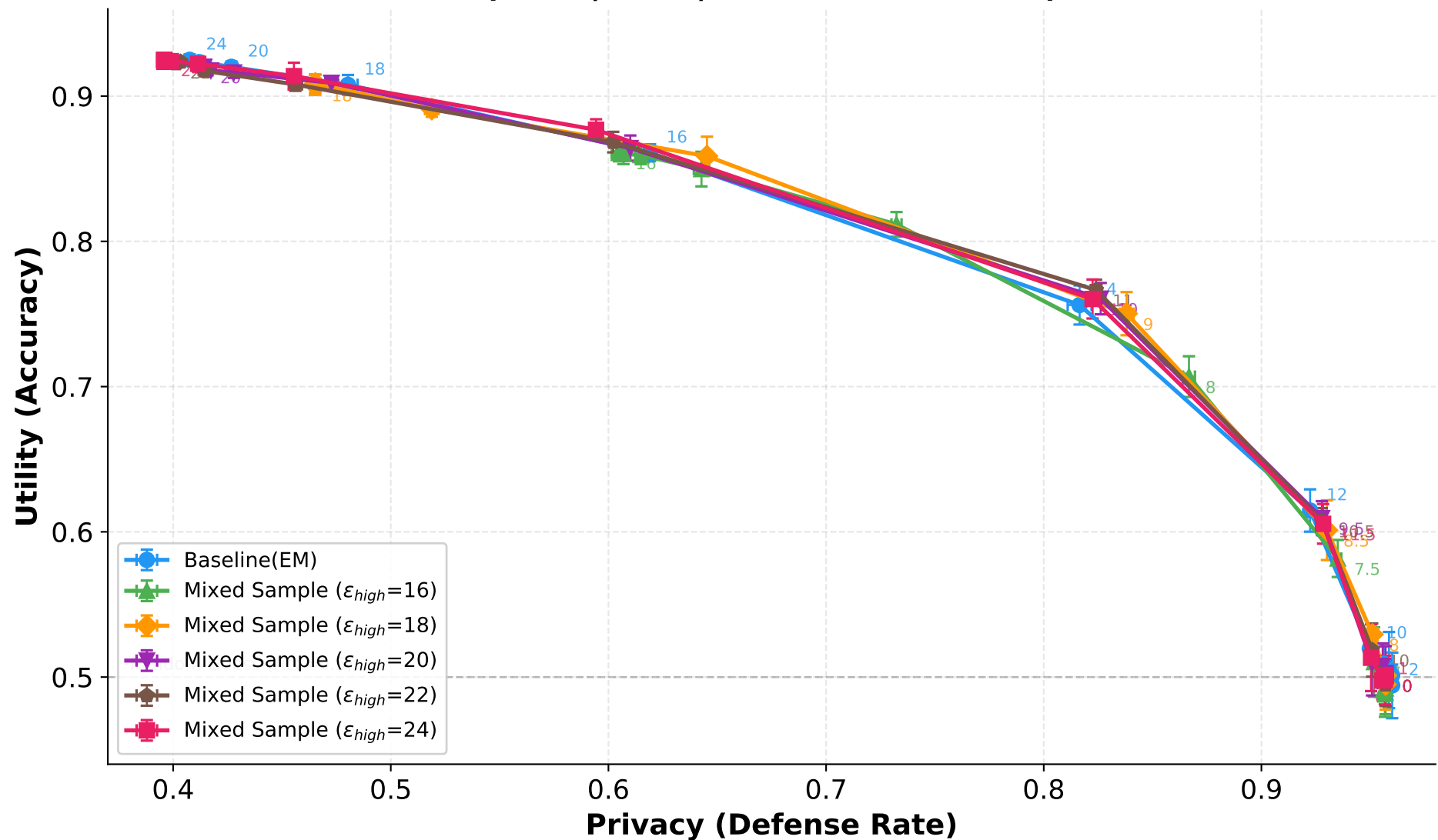
(SST-2, BERT, Mask Token Attack)
