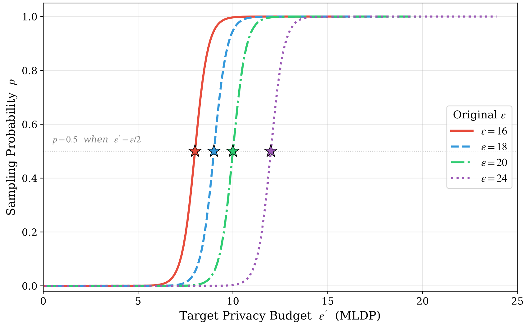
Sample Amplification: p vs \epsilon'
