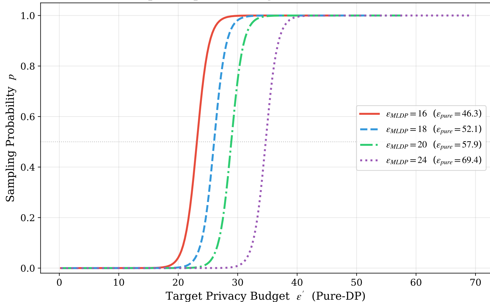
Sample Amplification: p vs \epsilon' (Pure-DP scale)
