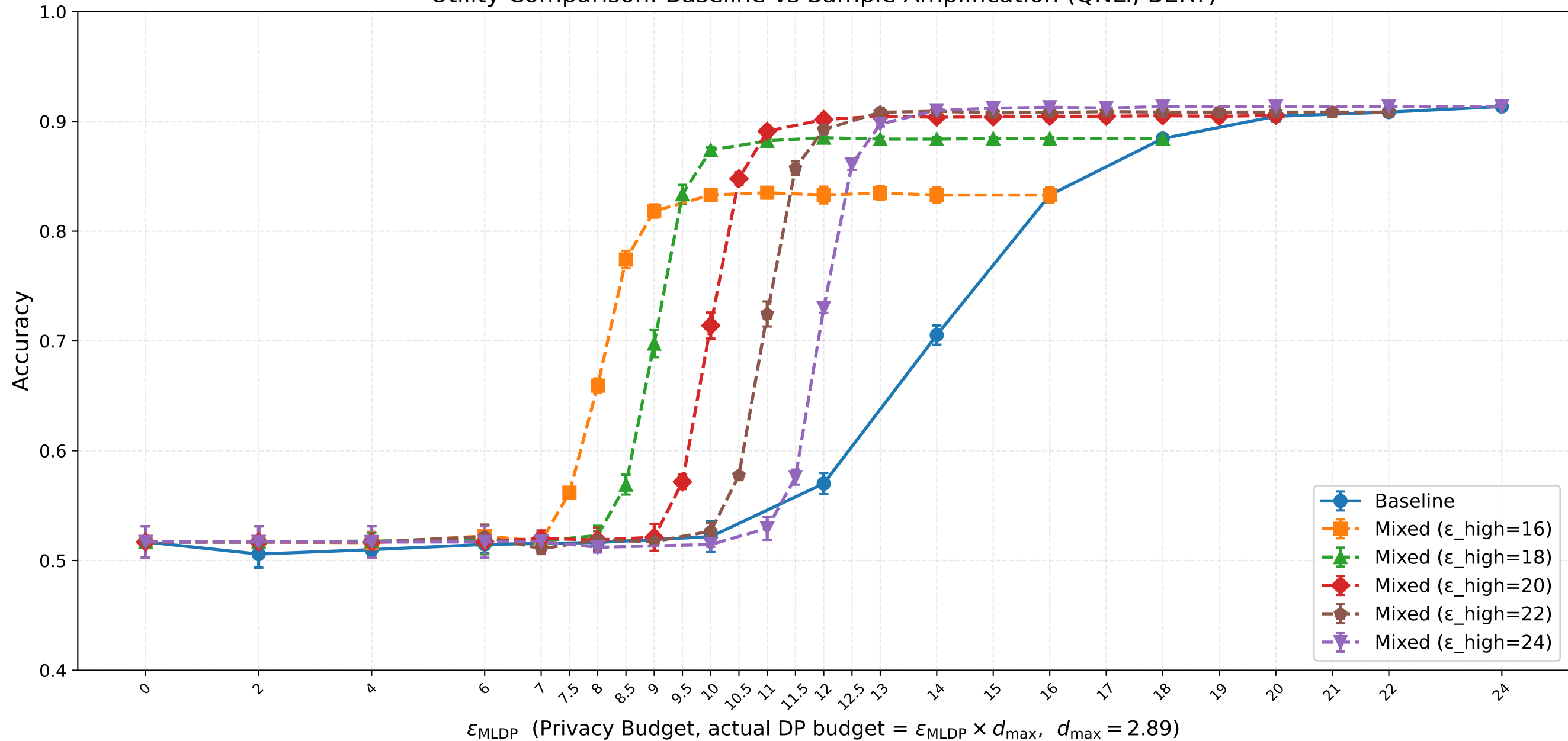
Utility Comparison: Baseline vs Sample Amplification (QNLI, BERT)
