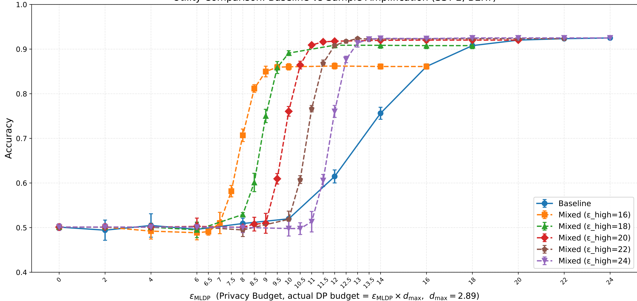
Utility Comparison: Baseline vs Sample Amplification (SST-2, BERT)
