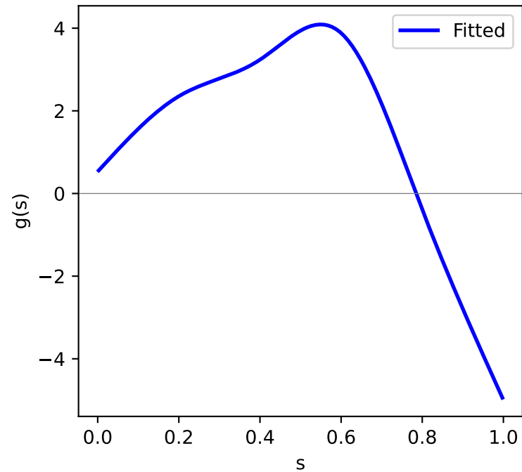
Net Growth
