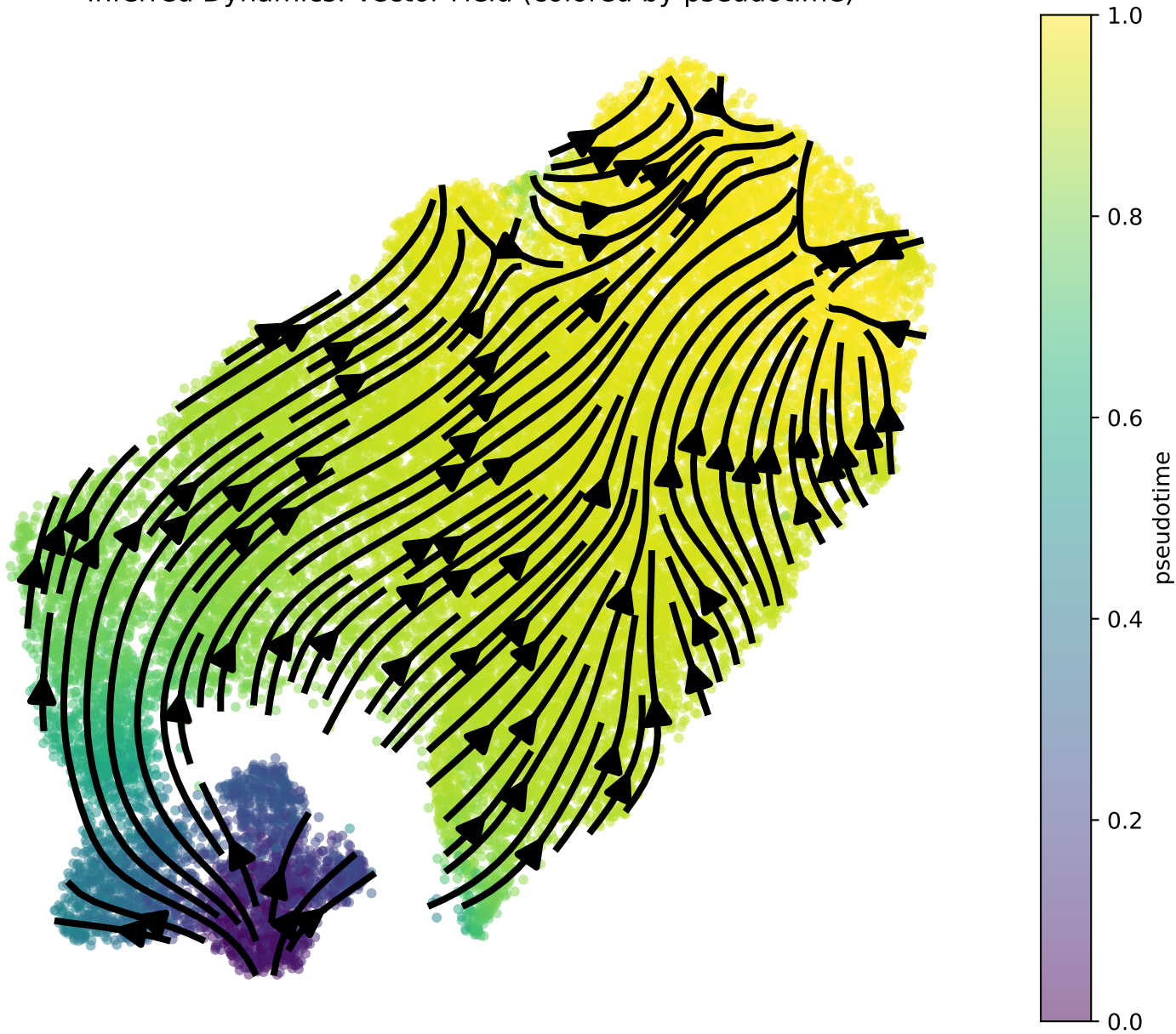
Inferred Dynamics: Vector Field (colored by pseudotime)
