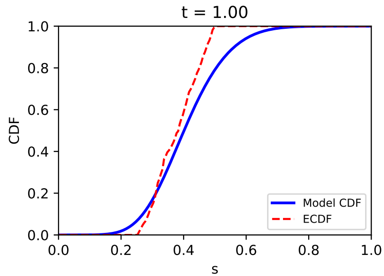
ECDF vs Model CDF
