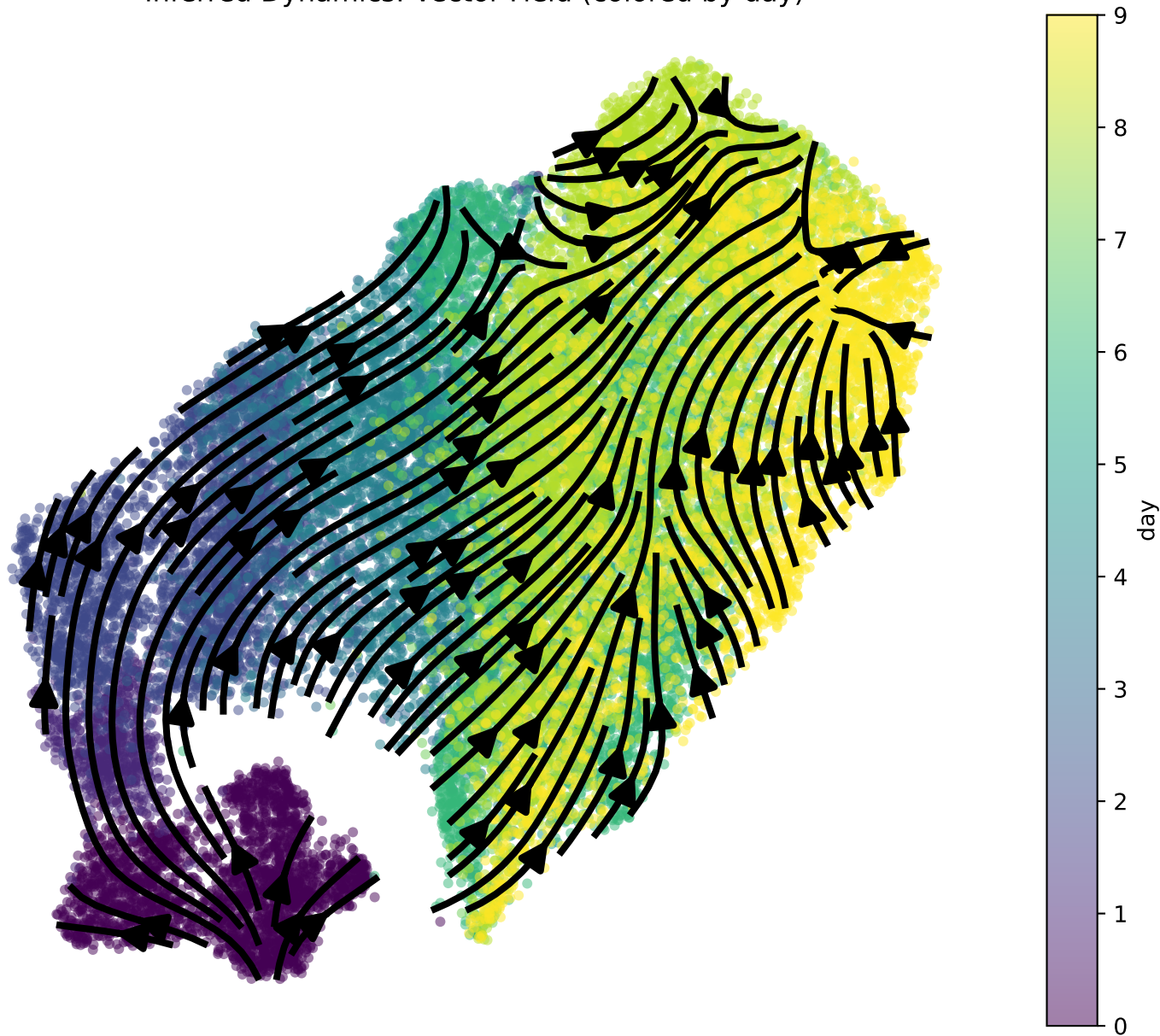
Inferred Dynamics: Vector Field (colored by day)
