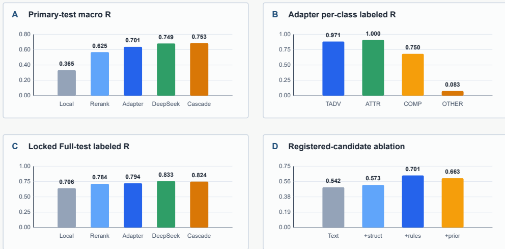
Figure 3. Composite performance view: (A) Primary-test macro labeled recall for the local model, train-only reranker, flat-feature adapter, DeepSeek, and cascade; (B) per-class labeled recall for the final adapter; (C) locked Full-test robustness; and (D) the registered-candidate ablation and five-split stability summary. Values are reported in Tables 5-7.
