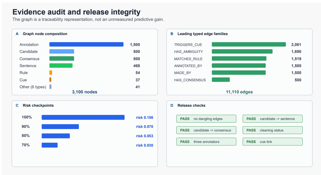
Figure 5. Public evidence audit: (A) graph node composition, (B) leading typed edge families, (C) locked risk-coverage checkpoints, and (D) six release-integrity checks. The graph is an auditable representation and is not treated as a measured relational-model gain.
