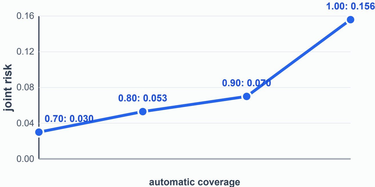
Risk-coverage curve
