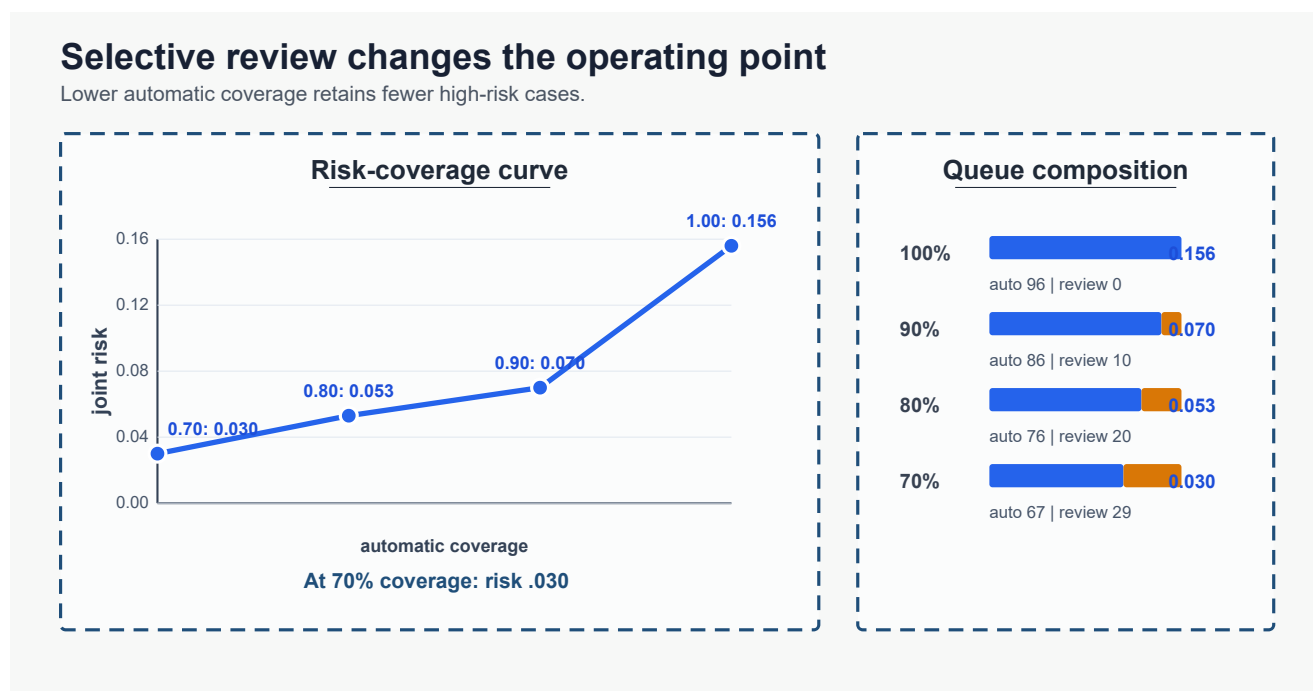
Figure 3. Selective routing lowers retained joint risk as automatic coverage decreases. The 70% operating point routes 29 of 96 registered keys and retains .030 joint risk. Source: locked routing table in the CAIT full-author manuscript.
