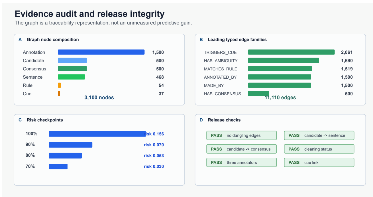
Figure 5. Public evidence audit: (A) graph node composition, (B) leading typed edge families, (C) locked risk-coverage checkpoints, and (D) six release-integrity checks. The graph is an auditable representation and is not treated as a measured relational-model gain.
