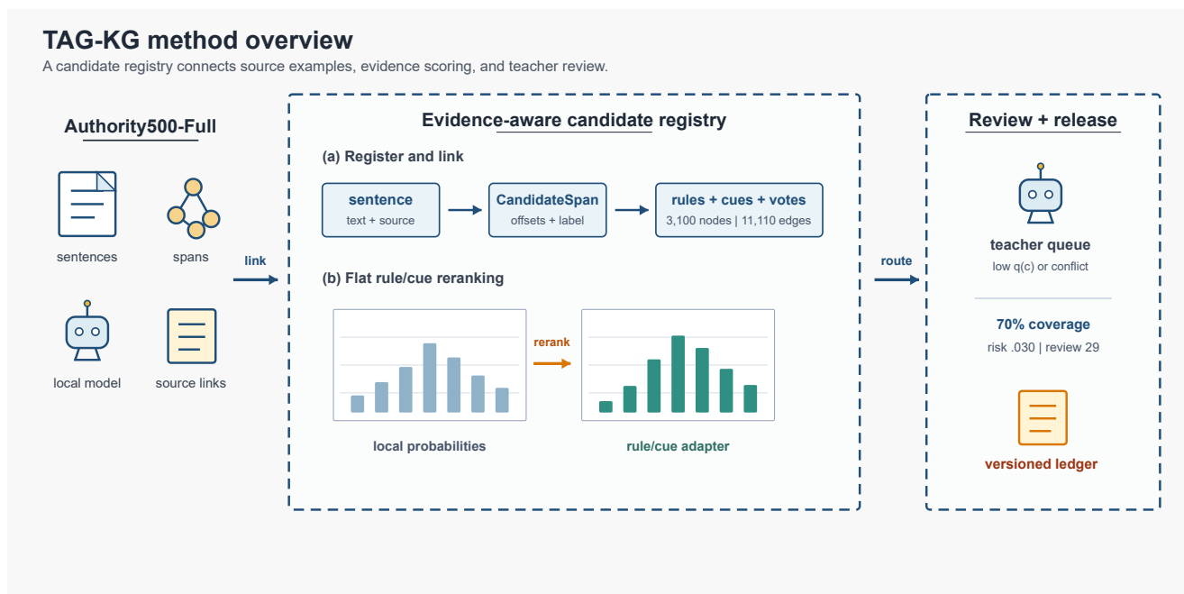
Figure 1. TAG-KG separates evidence-aware prediction, candidate-centric representation, and teacher review with versioned feedback. The flat rule scorer affects predictions; graph topology supports retrieval, provenance, and audit rather than supplying an unmeasured relational-model gain. Source: architecture contract in the CAIT full-author manuscript.
