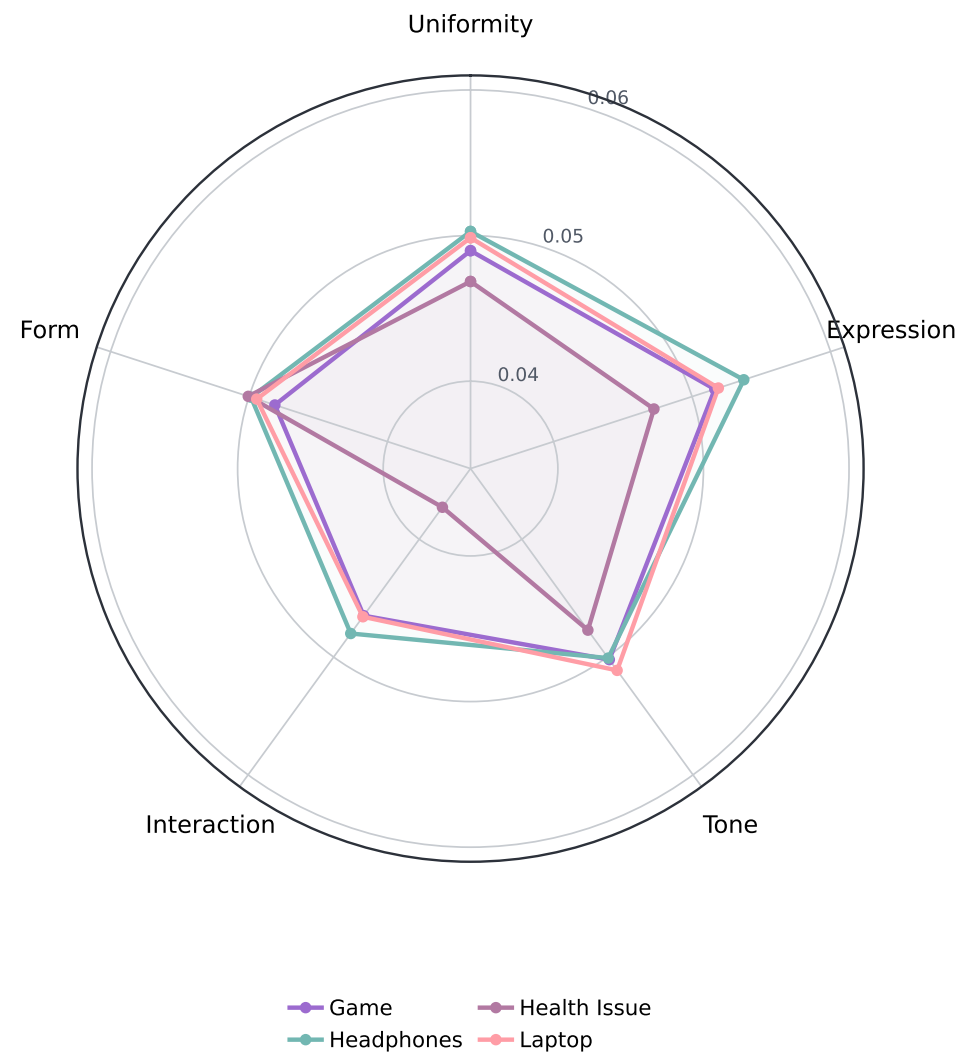
Raw family-mean |Cliff's delta|
