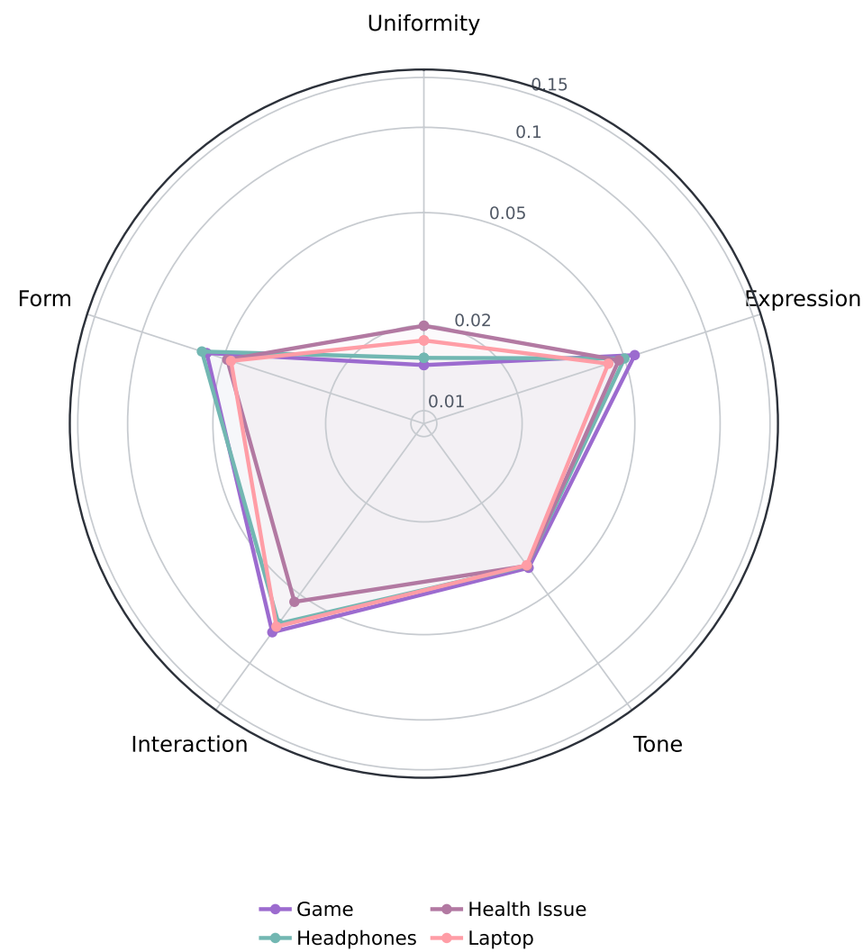
Raw family-mean Wasserstein distance
