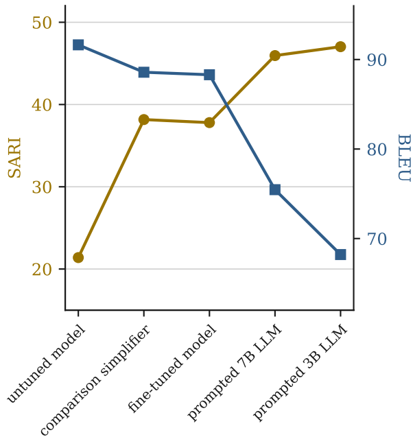
(a) Conditions ordered by BLEU
