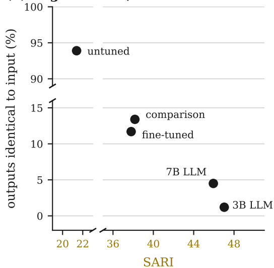
(b) Higher SARI, fewer unedited outputs
