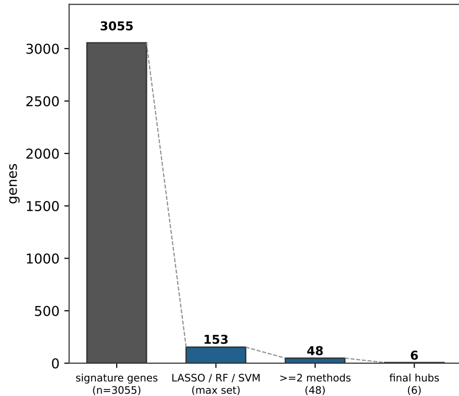
B. ML triple-filter convergence (G3 PASS)
