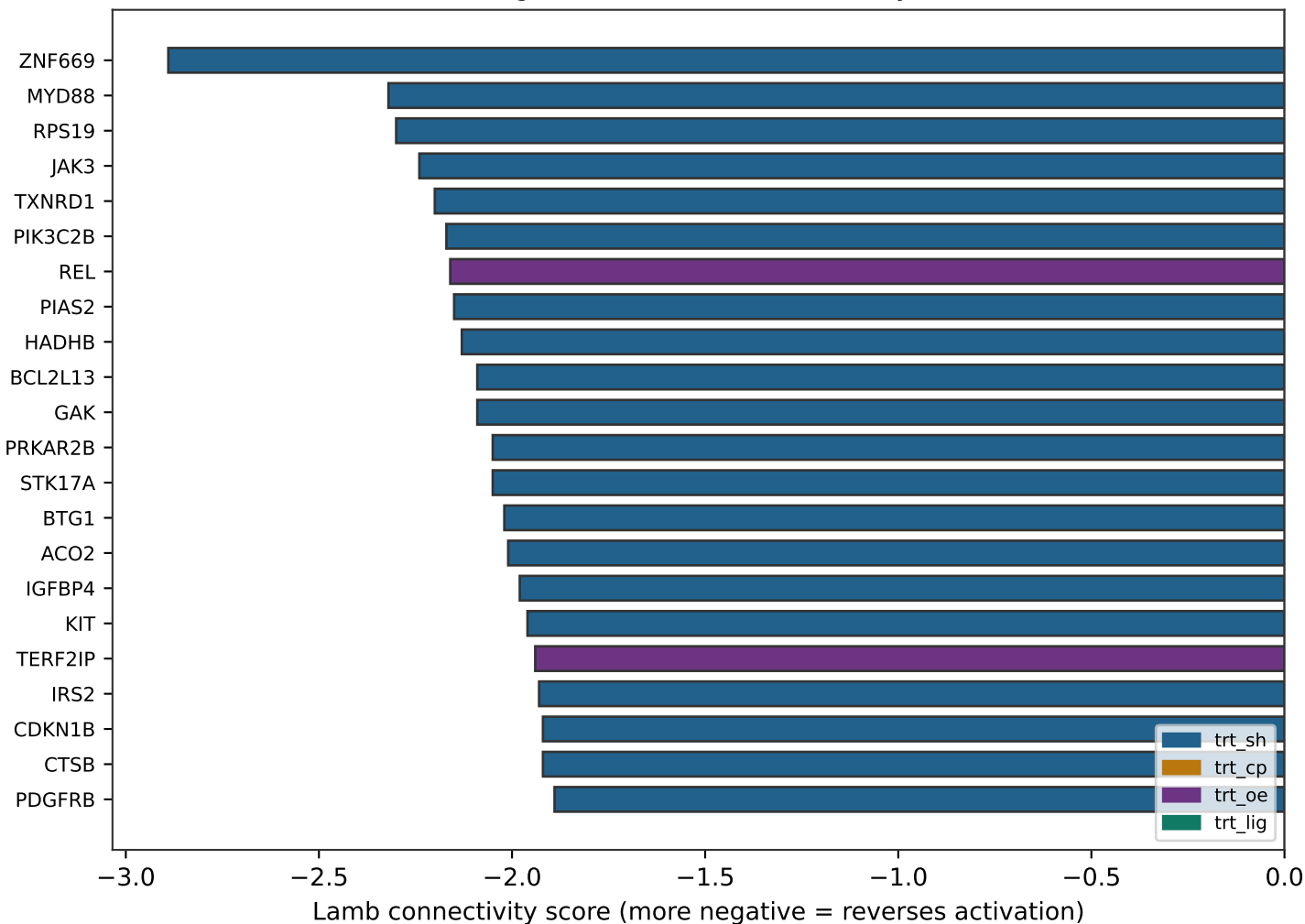
Top LINCSeq perturbations reversing the NP-activation signature (convergent NF- \kappa B / innate-immunity axis)
