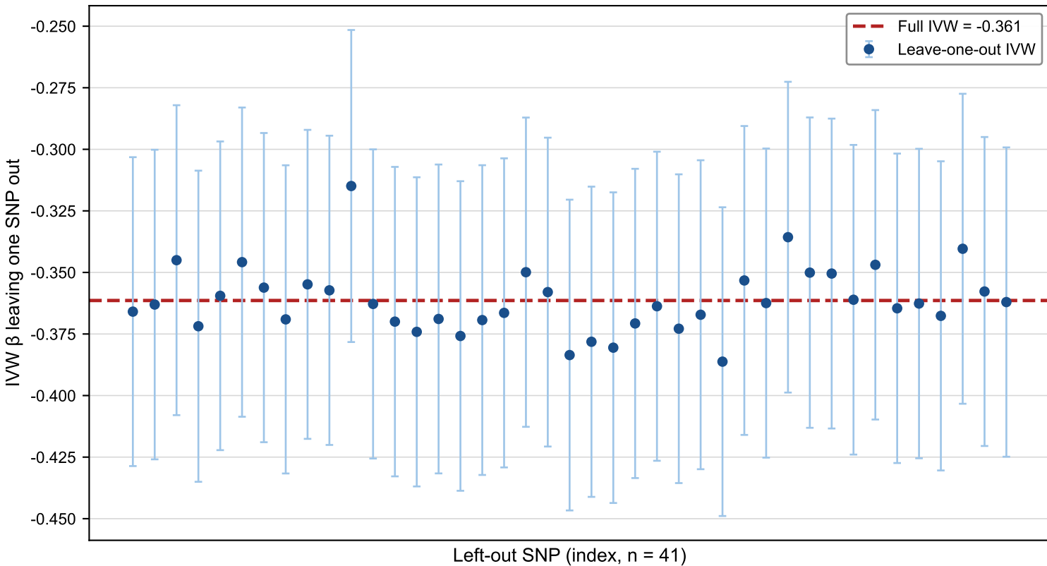
Figure 6. Leave-one-out sensitivity analysis (MCP → cognition)
