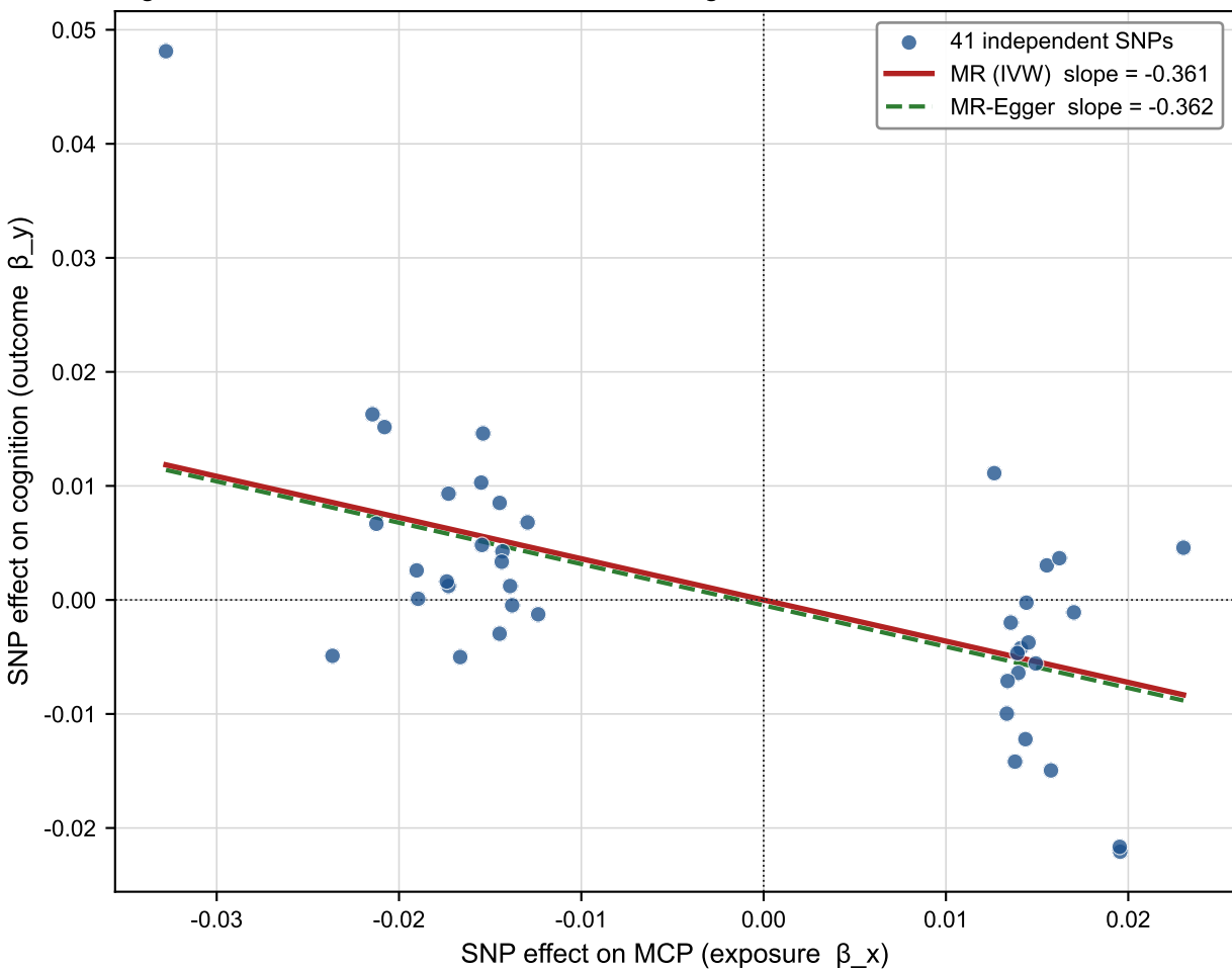
Figure 5. SNP-level associations: MCP \rightarrow cognition
