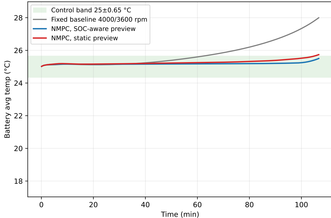
Peak shaving S0: constant 560 A discharge (6400 s)
