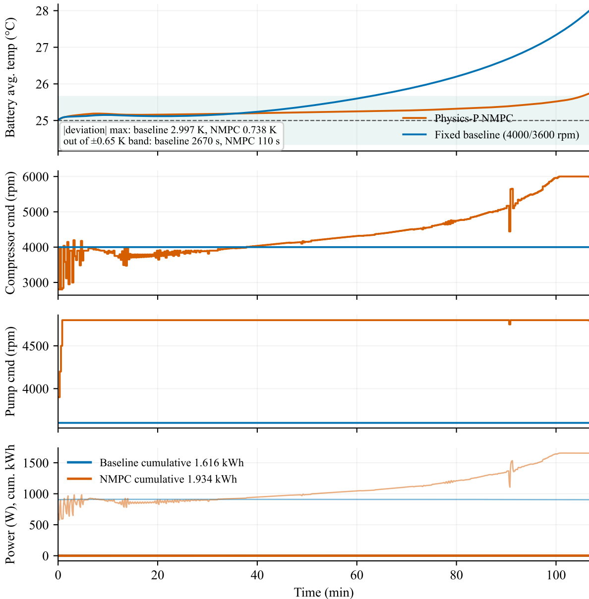
Peak-shaving S0, 560 A constant discharge over 6400 s (1280 steps)
