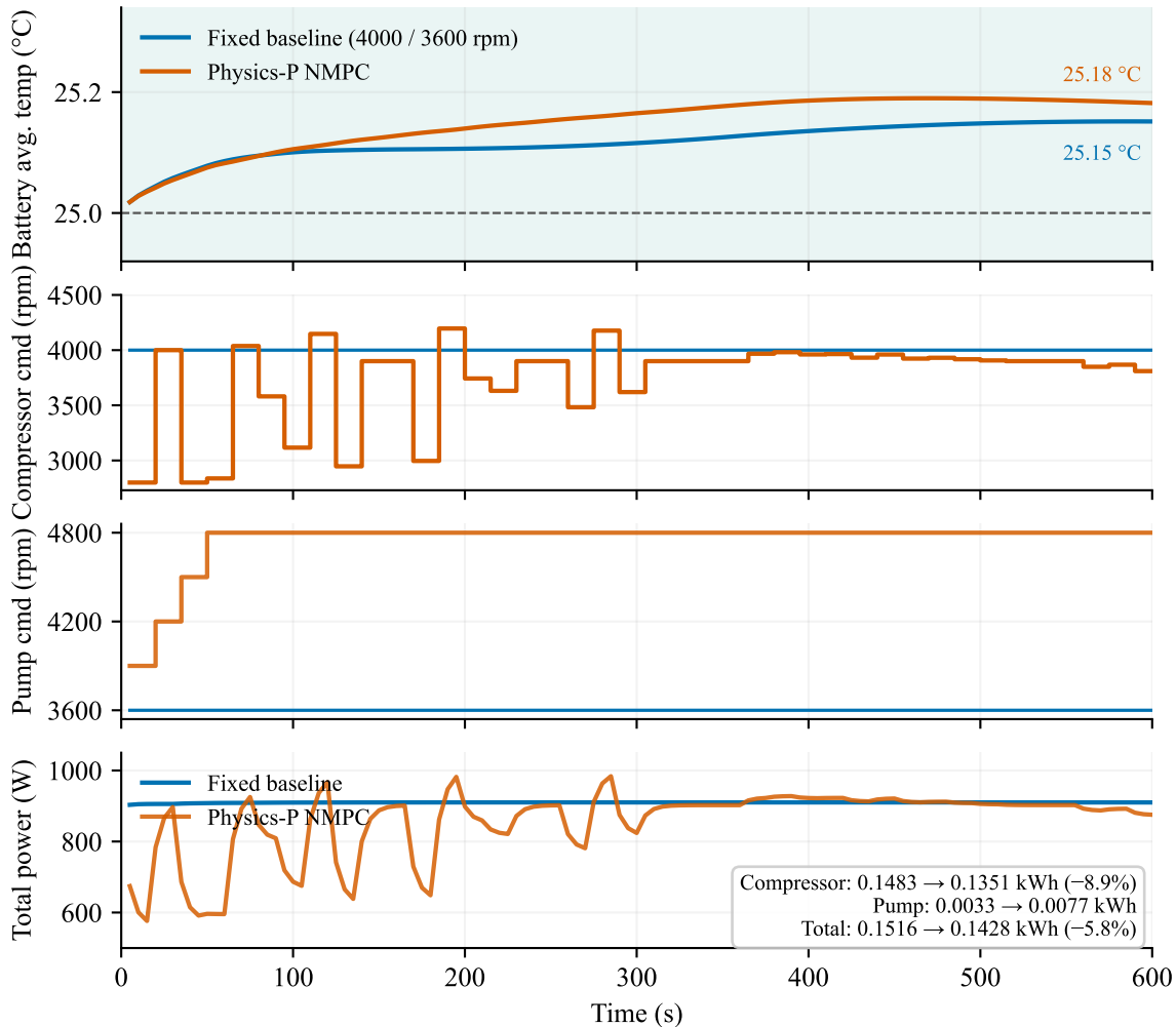
Peak-shaving case S0: 560 A constant discharge, 600 s (target 25\text{ }^{\circ}\text{C} \pm 0.65\text{ K} )
