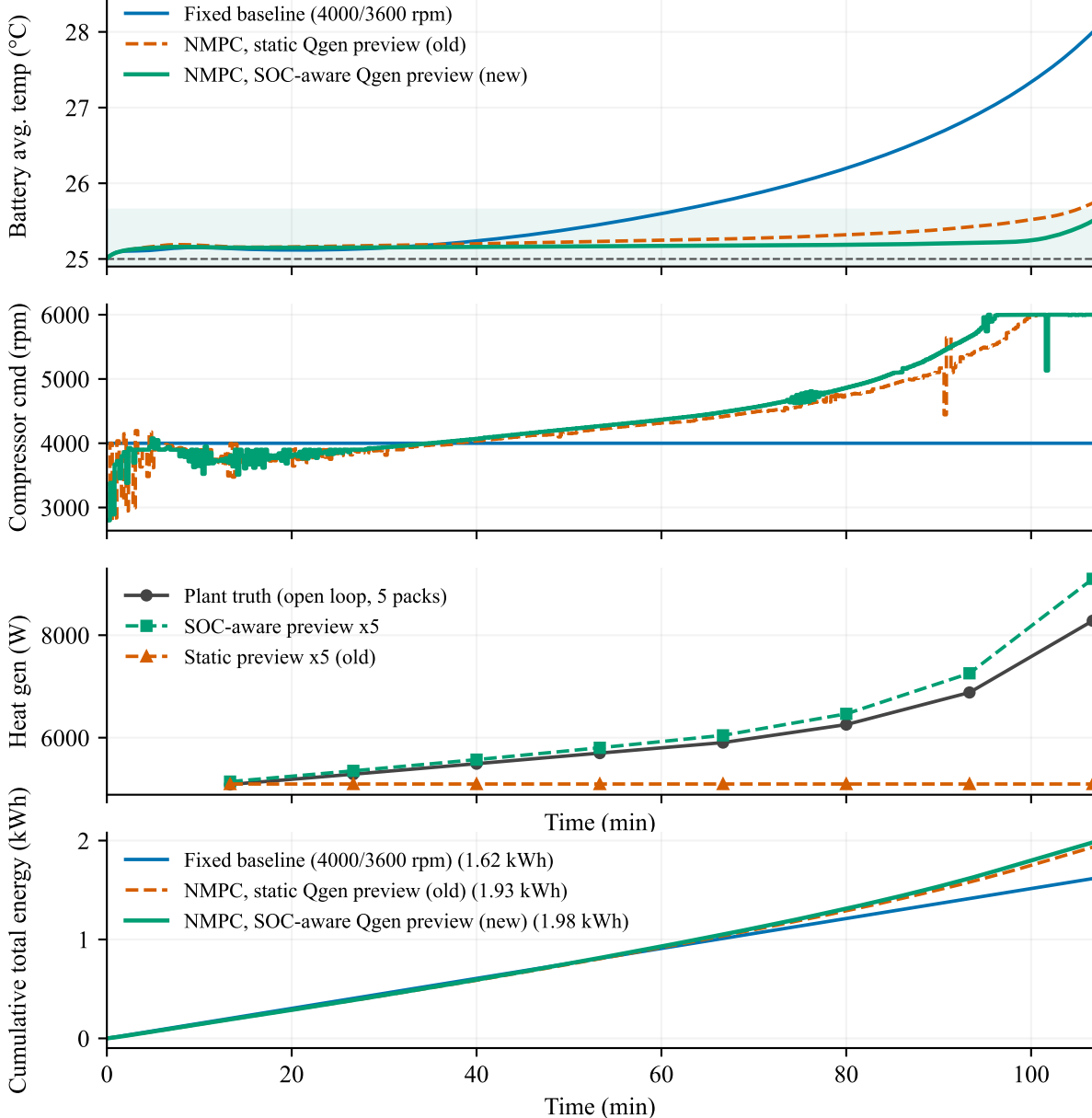
Peak-shaving S0 1280 steps: SOC-aware vs static Qgen preview
