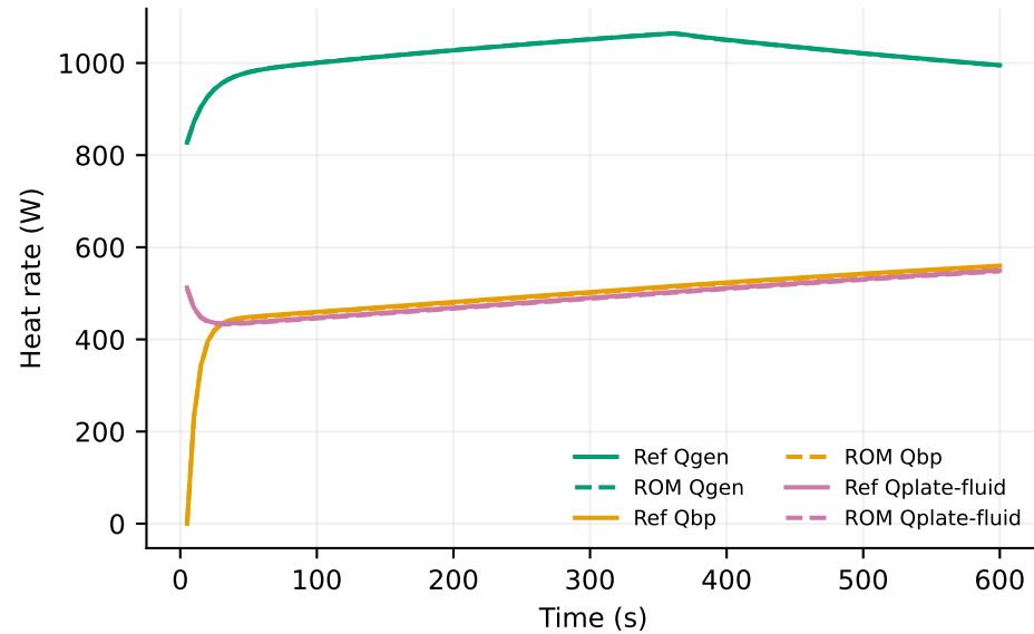
Heat-transfer rates
