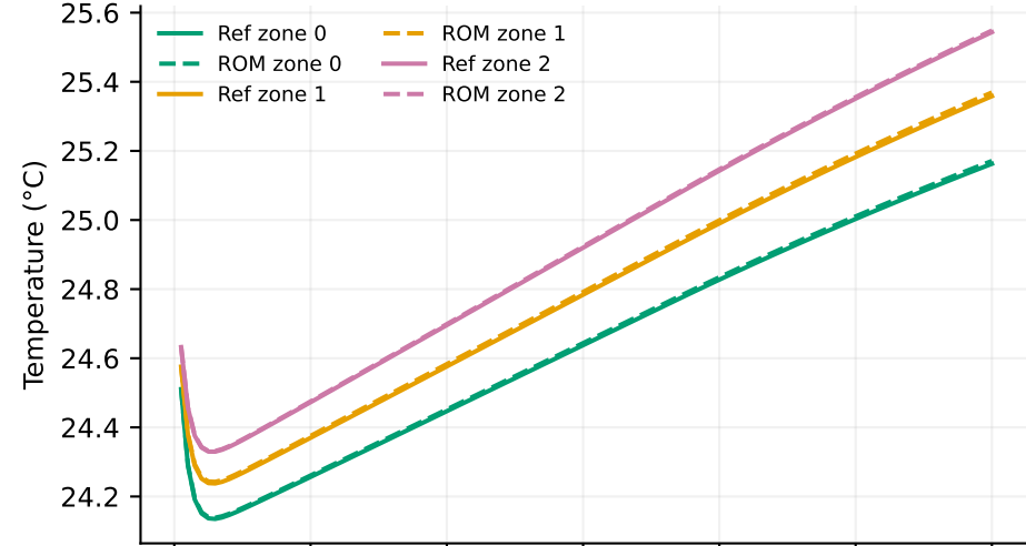
Cold-plate zone temperatures
