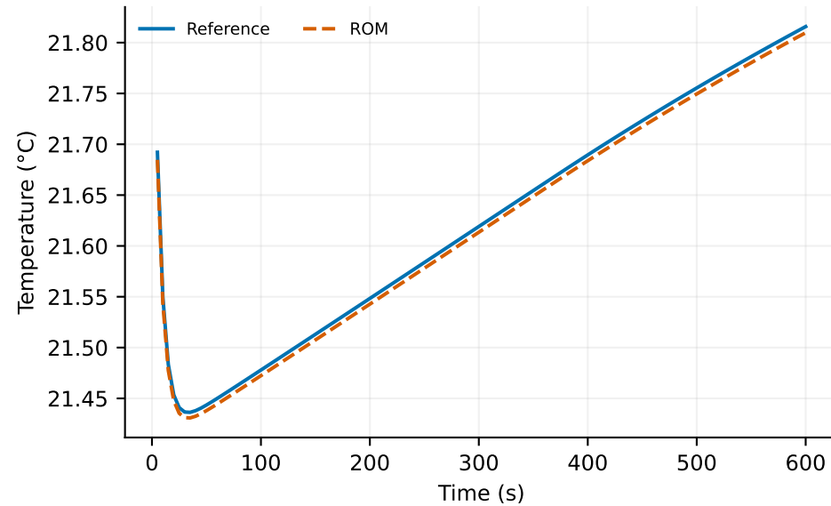
Coolant outlet
