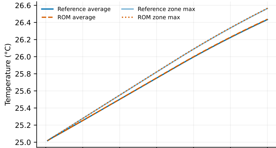
Battery temperatures
