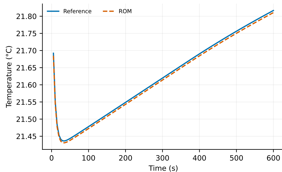
Coolant outlet
