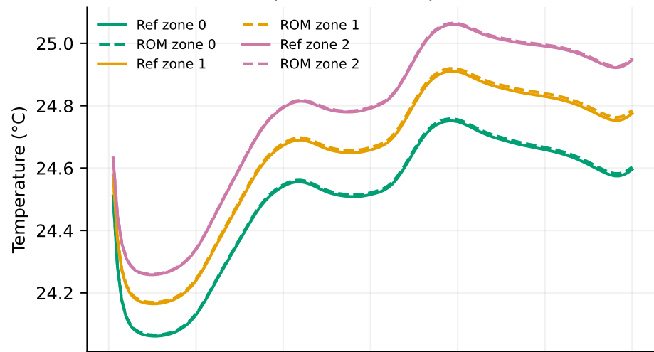
Cold-plate zone temperatures
