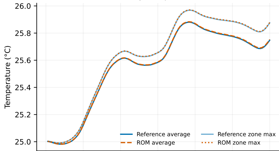
Battery temperatures
