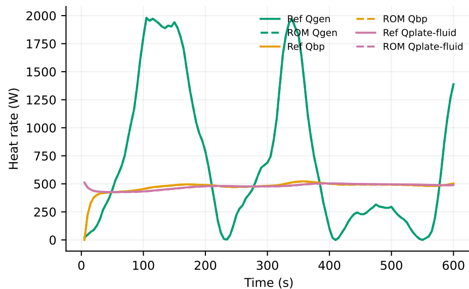
Heat-transfer rates
