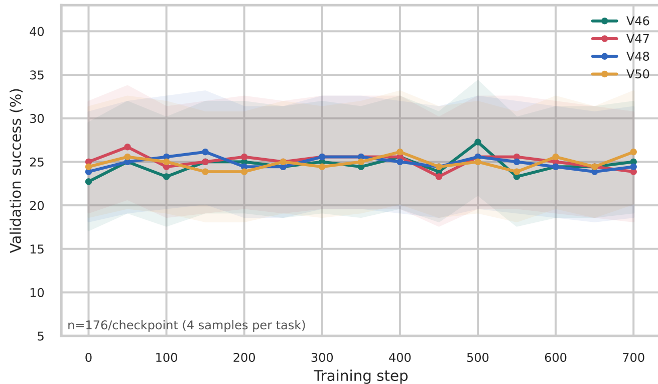
Qwen clean variants
