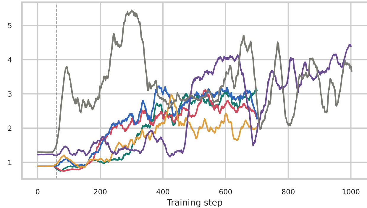
Policy entropy, MA(25)
