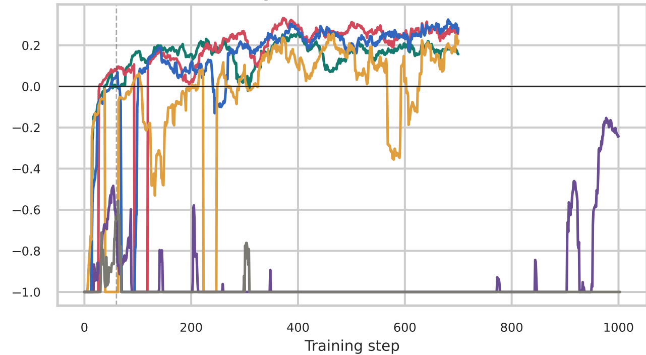
Critic explained variance, MA(25)
