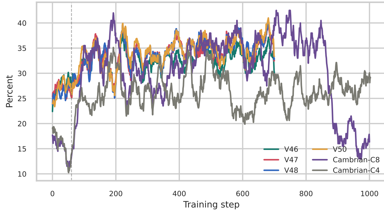
Train success, MA(25)
