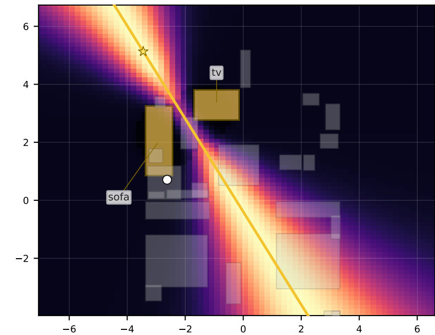
Equidistance Move to any position equidistant from tv and sofa
