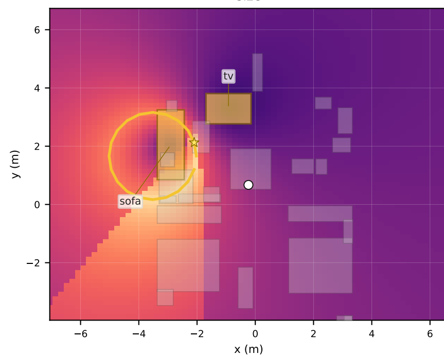
Size-distance invariance Position where tv and sofa appear same size
