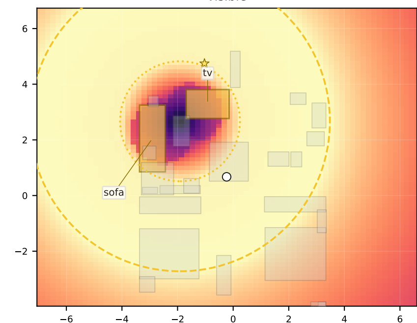
FoV inclusion Position where both tv and sofa are visible
