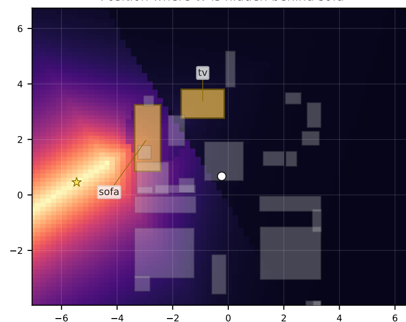
Occlusion alignment Position where tv is hidden behind sofa
