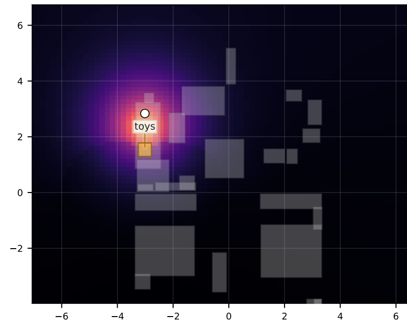
Look-at heading, geometric score. Gray boxes are other furniture. Delta control Move 0.5m toward toy_animals
