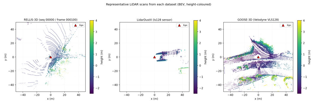
Figure 6. Representative LiDAR scans from each dataset, projected to BEV and coloured by height (clip range -2.5 m to +4.0 m). (a) RELLIS-3D — vegetation-heavy off-road, Ouster OS1-64 ( \sim 37 k points/scan). (b) LidarDustX — dusty construction environment, multi-sensor capture ( \sim 111 k points/scan with the LS128 sensor shown). (c) GOOSE-3D — mixed European outdoor (forests, fields, campus), Velodyne VLS128 ( \sim 199 k points/scan). The red triangle marks the ego vehicle.
