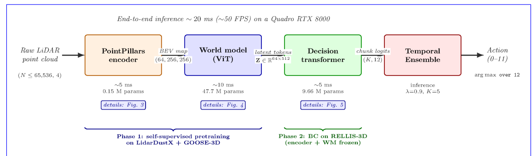
Figure 2. High-level dataflow of TerrainFormer. A raw LiDAR point cloud (left) passes through four stages : the PointPillars encoder to produces a 64 \times 256 \times 256 BEV feature map, which the ViT-based world model compresses it to 64 latent tokens \mathbf{Z} \in \mathbb{R}^{64 \times 512} , the decision transformer attends jointly to these tokens, an action-history buffer, and a learnable produces (K, 12) chunk query logits, and predicts K=5 future actions . Temporal Ensemble (right) averages/aggregates overlapping chunks for jitter-free outputs across the last K=5 frames into a single discrete action. Block-internal details are deliberately omitted here . Component internals are deliberately omitted here and are shown in expanded views: encoder (in Fig. 3 (encoder)), world model (Fig. 4 (world model)), and decision transformer (Fig. 5 (decision transformer)). Symbol legend Per-stage latency and parameter counts are annotated below each block; total end-to-end inference is \sim 20 ms ( \sim 50 FPS) on a Quadro RTX 8000. Bottom braces show the two-phase training schedule: B -batch encoder + world model pretrained self-supervised on LidarDustX + GOOSE-3D (Phase 1, N -points/scan blue), H \times W = 256 \times 256 BEV cells then frozen while the decision transformer is trained with behavioral cloning on RELIS-3D (Phase 2, d=512 -embedding, K=5 -chunk, A=12 -actions green).
