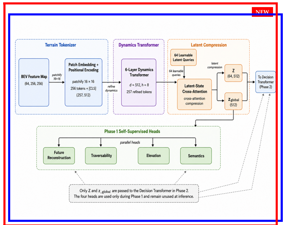
Figure 4. Component view of the world model. The three internal modules (terrain tokenizer, dynamics transformer, latent compression) and the four self-supervised heads used during Phase 1 pretraining are shown explicitly. Only \mathbf{Z} (64 latent tokens) and \mathbf{z}_{\text{global}} are passed on to the decision transformer in Phase 2; the four prediction heads remain unused at inference and after Phase 1 the entire world model is frozen.
