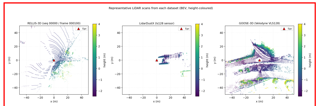
Figure 6. Representative LiDAR scans from each dataset, projected to BEV and coloured by height (clip range -2.5 m to +4.0 m). (a) RELLIS-3D — vegetation-heavy off-road, Ouster OS1-64 ( \sim 37 k points/scan). (b) LidarDustX — dusty construction environment, multi-sensor capture ( \sim 111 k points/scan with the LS128 sensor shown). (c) GOOSE-3D — mixed European outdoor (forests, fields, campus), Velodyne VLS128 ( \sim 199 k points/scan). The red triangle marks the ego vehicle.
